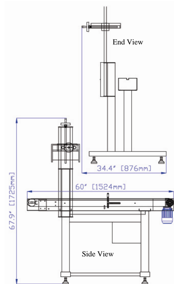
Dimensional Drawing
