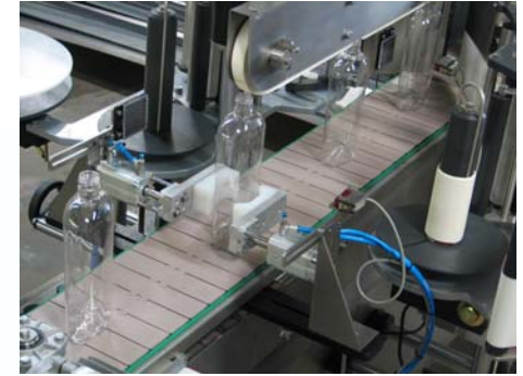
Stepper Pneumatic In Feed Module For Increased Label Placement Accuracy with Oval or Angled Surfaces
