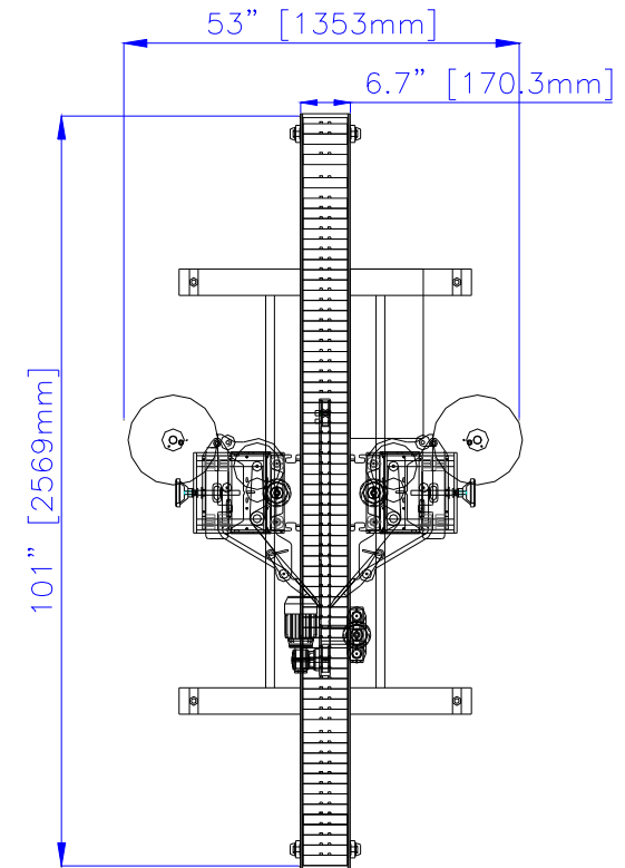
Dimensional Drawing
