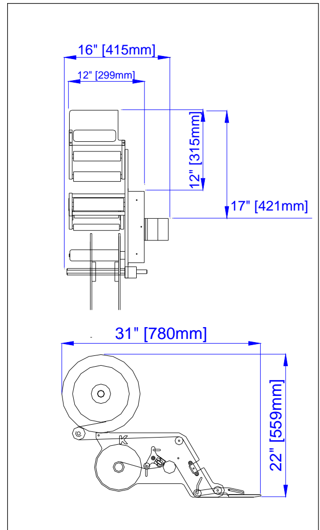
Dimensional Drawing
